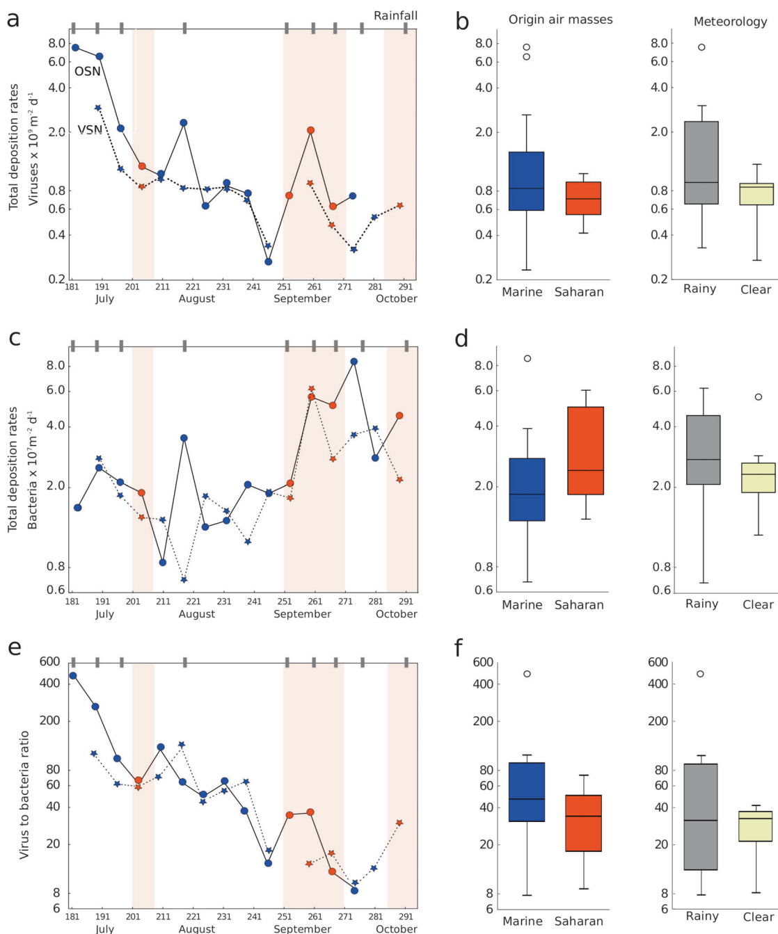
Fig. 3 Synchronous dynamics of total (dry + wet) deposition rates of a viruses, c bacteria, and e virus-to-bacteria ratios at the Observatory (OSN) (circles) and Veleta Peak (VSN) in Sierra Nevada, Spain. Gray marks on the top axis indicate rain events. Samples that are predominantly marine in origin are shown in blue and samples that are
